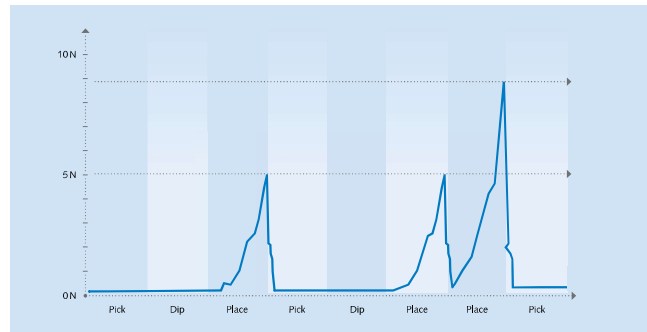
Graphic view of a pick- and-place application showing the force curve for removing and placing the dies
